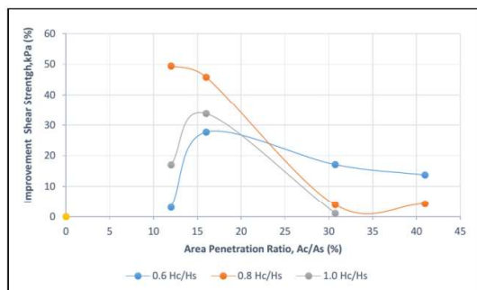
Fig. 7 Improvement Shear Strength versus Area Replacement Ratio
