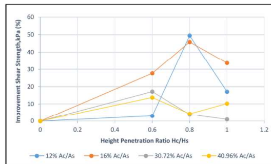
Fig. 8 Improvement Shear Strength versus Height Penetration Ratio
