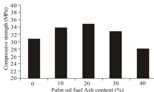
Fig. 3: Compressive strength of oil palm shell lightweight aggregate containing various palm oil fuel ash content at 28 days
