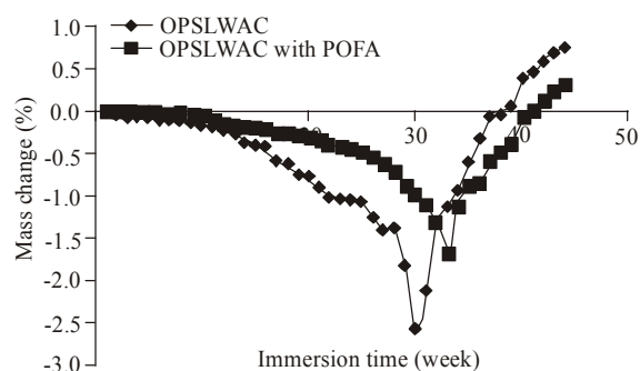
Fig. 4: Mass change of oil palm shell lightweight aggregate specimens after immersed in sodium sulphate solution for 45 weeks
