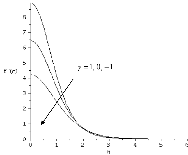
Figure 1: Velocity profiles when N_R = 10 and \xi = \infty (MBC case).
