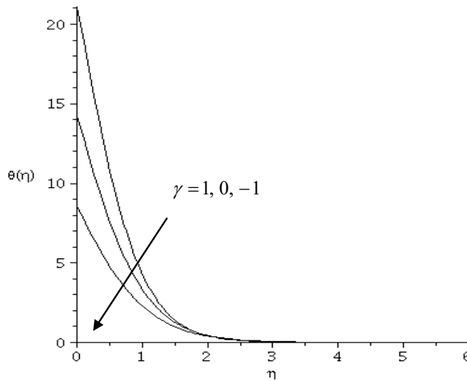
Figure 2: Temperature profiles when N_R = 10 and \xi = \infty (MBC case).
