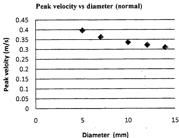
Figure 7: Peak velocity vs diameter for normal case
