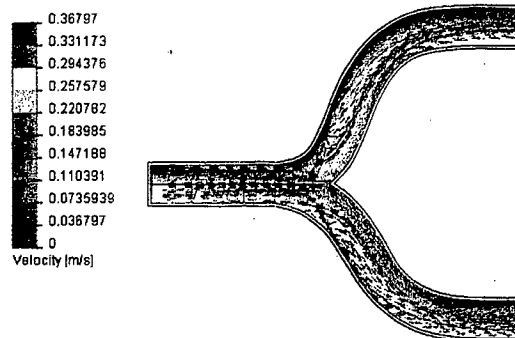
Figure 1: Velocity distribution for normal blood vessel
