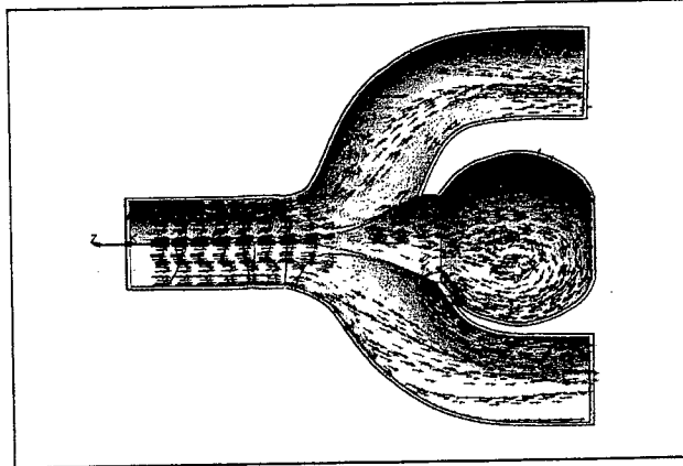
Figure 13: Velocity flow for diameter 14mm
