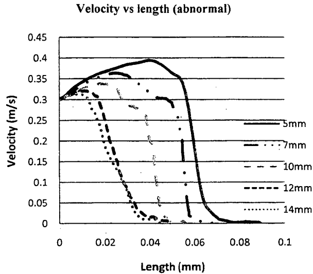
Figure 6: Graph velocity vs length for different diameter in abnormal case
