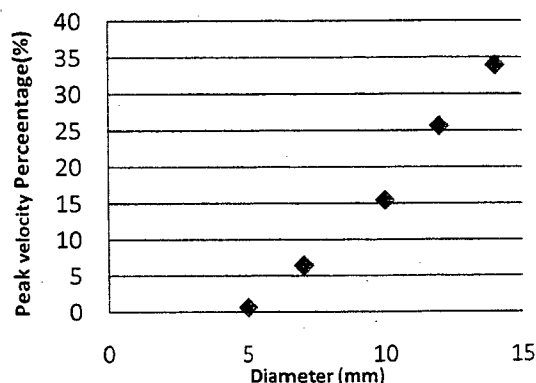
Figure 14: Graph percentage peak velocity different vs diameter
