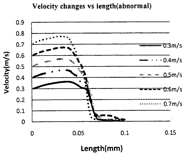
Figure 4: Graph velocity vs length for different velocity in abnormal case
