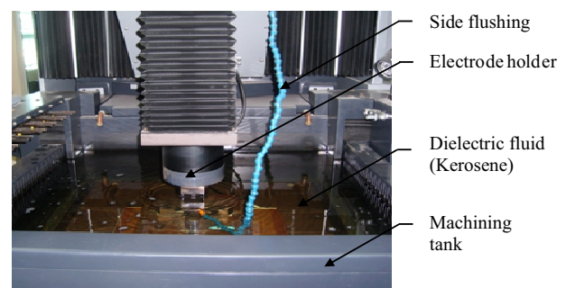
Fig. 2 Electrical discharge machining tank at operational state.
