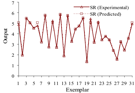
Fig. 6 Comparison between experimental and predicted output.
