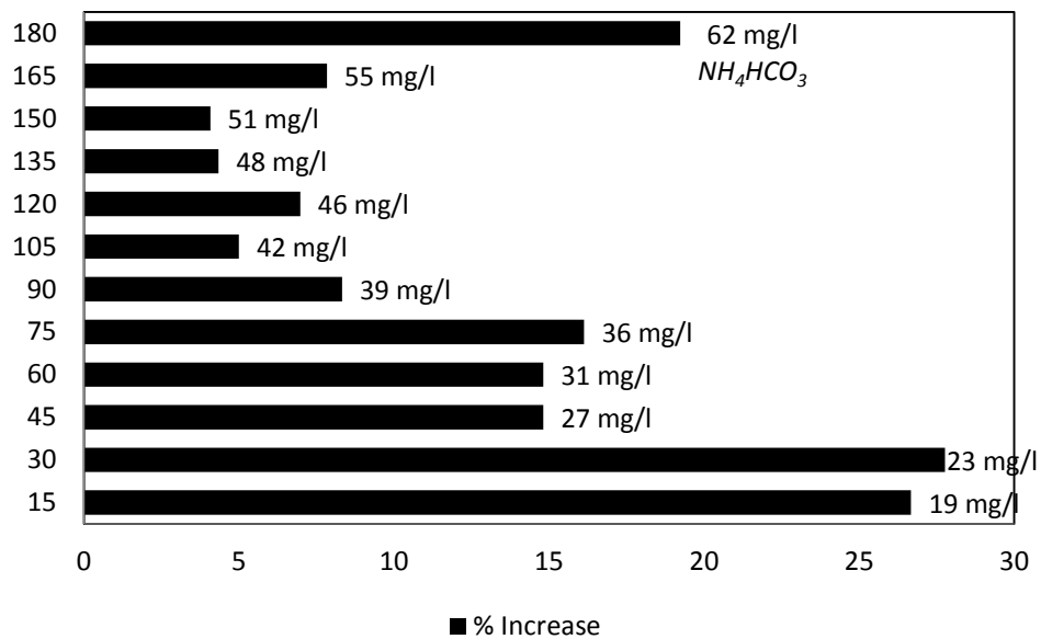
Figure 2 Determinations of % increase in biogas yield from NH_4HCO_3 supplemented co-digestion of PWW compared to control digestion of PWW
