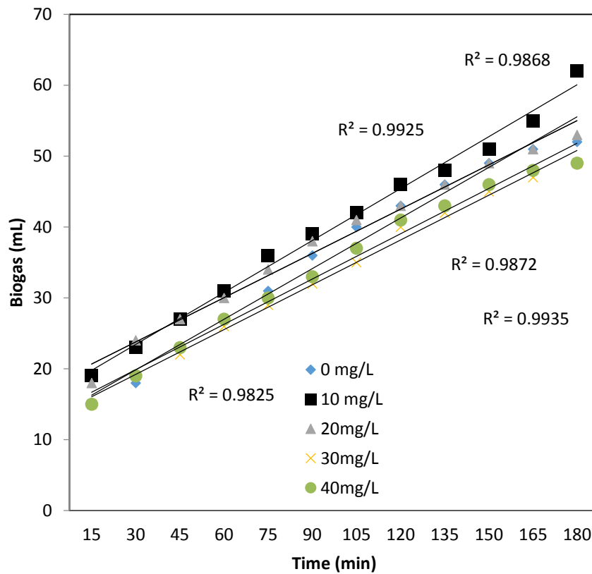
Figure 1 Evaluation of digestion performance in terms of cumulative biogas generation vs. time graph
