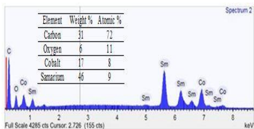
Fig. 7 EDX spectra of the used SmCoO 3 catalyst at feed ratio 1.0
