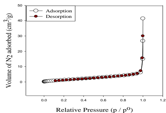
Fig. 2 \text{N}_2 physisorption isotherm of \text{SmCoO}_3 perovskite Catalyst
