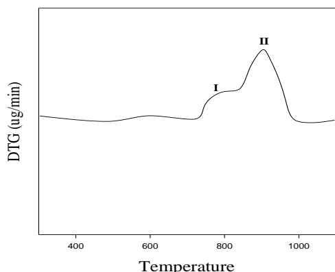
Fig. 8 TPO profile of the used SmCoO 3 perovskite catalyst at feed ratio 1.0.
