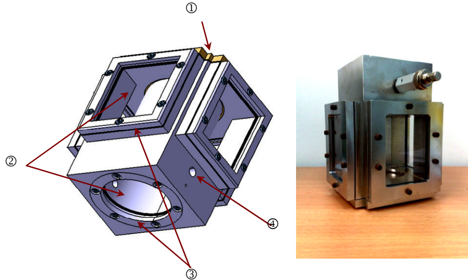
Figure 2: High-pressure chamber with optical access. ①Injector port. ② Windows /Optical access. ③ Window Body. ④Fuel and pneumatic access.
