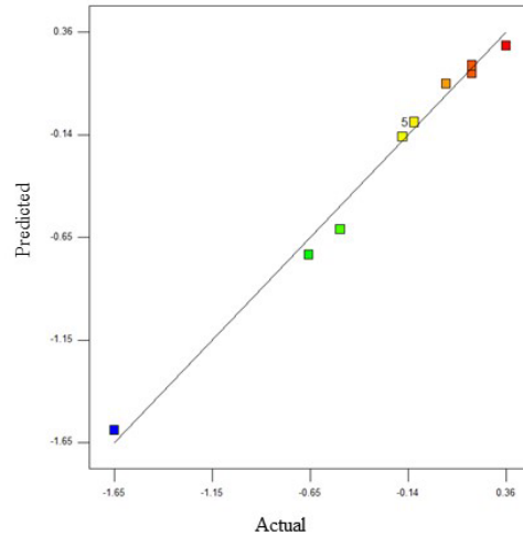
Figure 2. The comparison of predicted and experimental values for wax deposit amount using CCD
