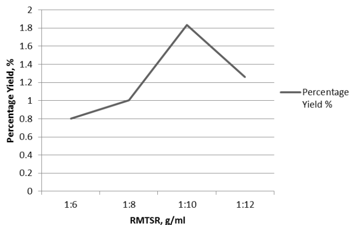
Fig. 3: Percentage Yield against RMTSR
