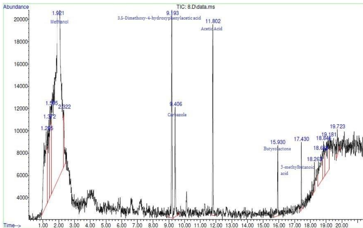
Fig. 5: GCMS of extract using Microwave Power of 200W.
