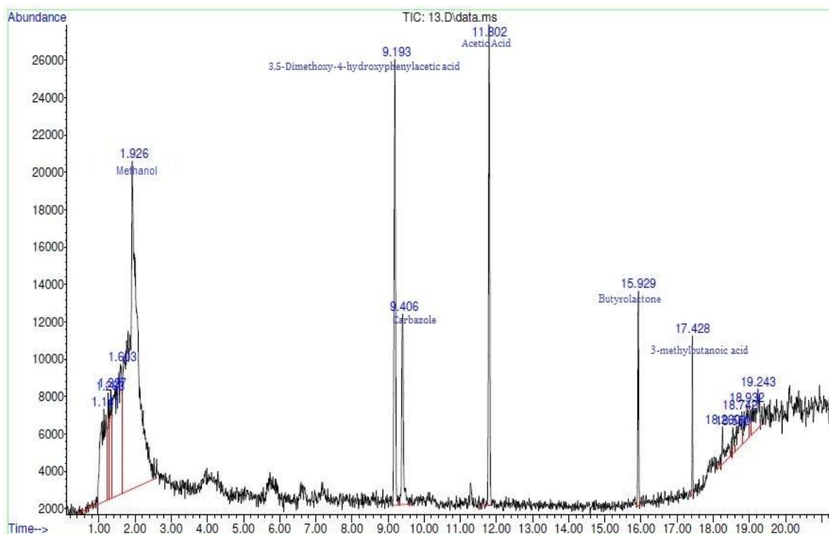
Fig. 6: GCMS extract weigh to solvent of 1:6.
