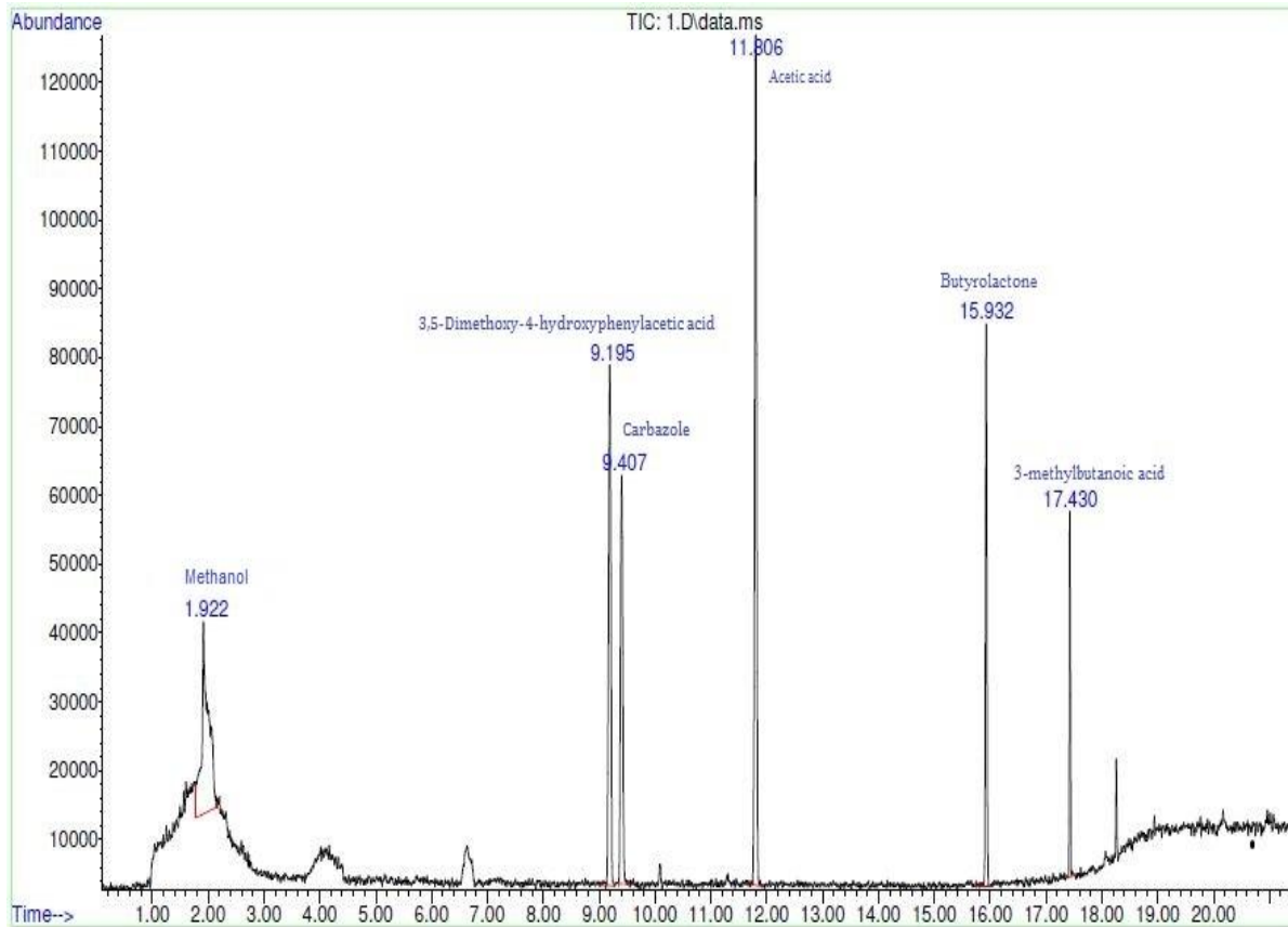
Fig. 4: GCMS of 5 minutes Extraction time.
