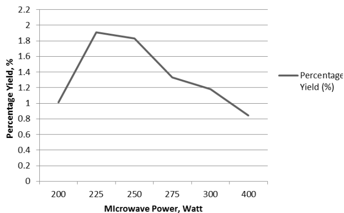
Fig. 2: Percentage Yield against Microwave Power.
