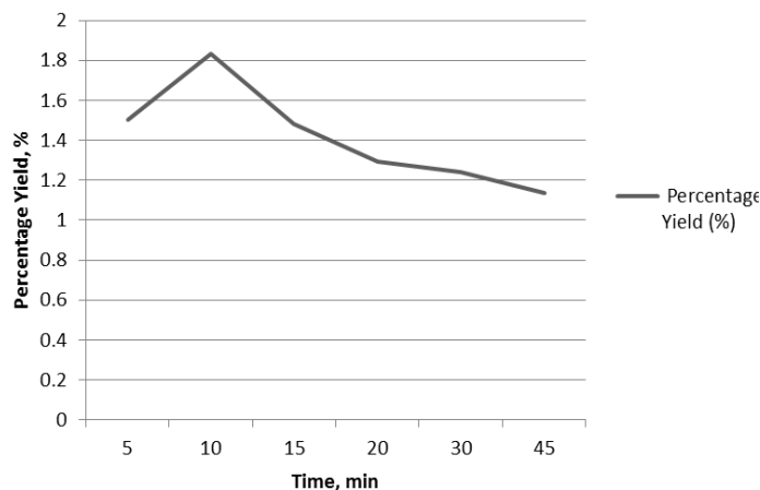
Fig. 1: Percentage Yield against Extraction Time.
