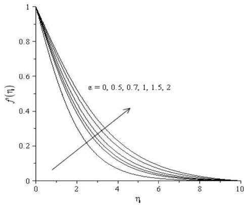
Fig. 3: Effect of \varepsilon on f'(\eta) when \delta = 2, \alpha = 1, \gamma = 0.005, \lambda = 0.5 and Pr = 0.7
