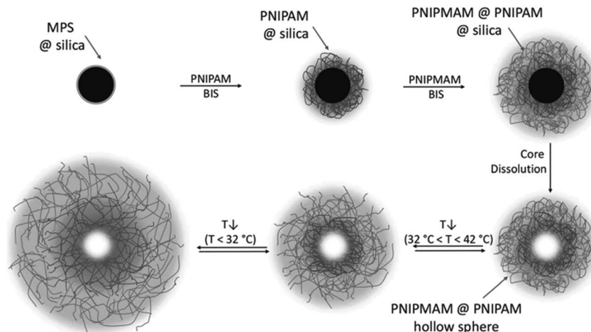
Fig. 8 Schematic of the synthesis process for doubly temperature-responsive core–double-shell microgels and hollow spheres. Reproduced from ref. 51 with permission from John Wiley and Sons.
