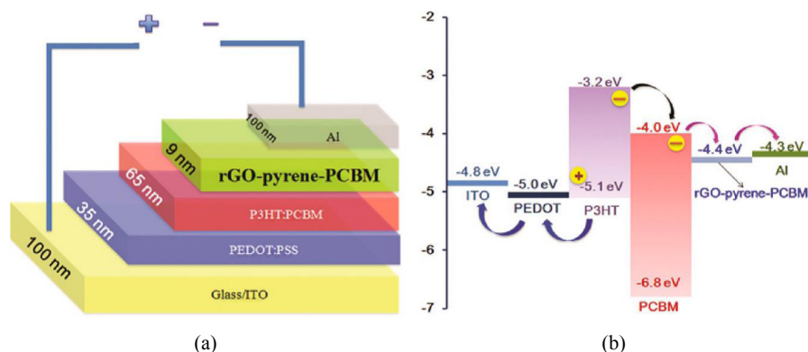
Figure 13 Schematic architecture, (a) energy level diagram (b) of ITO/PEDOT:PSS/P3HT:PCBM/RGO-PYRENE-PCBM/Al BHI-PSC device an incorporated RGO-pyrene-PCBM electron extraction layer (see online version for colours)
