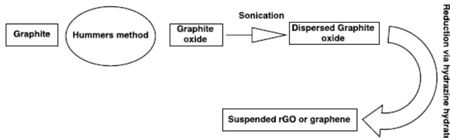
Figure 3 Schematic of the process flow mechanism for graphene synthesis derived from graphite
