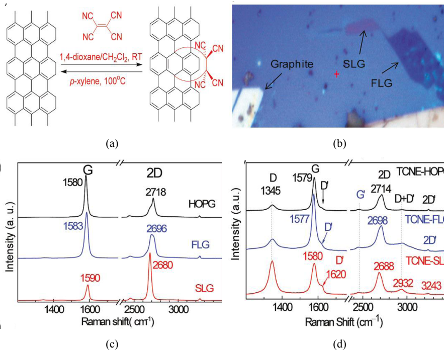
Figure 10 Room temperature Diels-Alder (DA) reaction between graphene (diene) and tetracyanoethylene (TCNE, dienophile) (see online version for colours)
