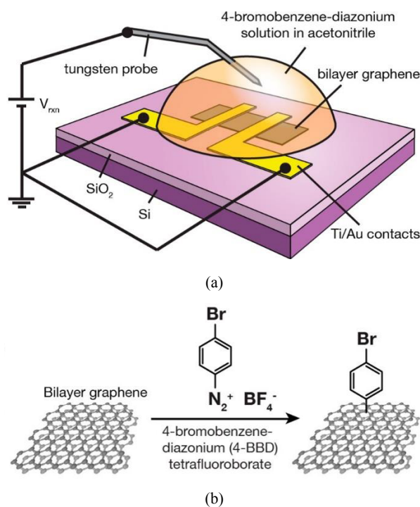
Figure 8 Covalent electrochemical functionalisation of two-layer grapheme, (a) schematic of the experimental setup. Two-layer graphene generated via mechanical exfoliation is on SiO 2 /Si wafer and is grounded via Ti/Au metal contacts. A droplet of 4-bromobenzene-diazonium (4-BBD) tetrafluoroborate solution in acetonitrile covers the two-layer flake. A tungsten probe is inserted into the solution droplet to apply a bias voltage during the reaction, V rxn (b) reaction scheme for the covalent modification of 4-BBD on bilayer grapheme (see online version for colours)
