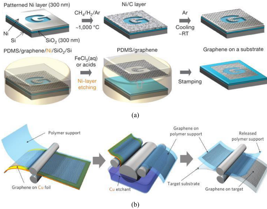
Figure 4 (a) Schematic of CVD preparation of graphene and transfer via polymer support, the carbon interfaces with the Ni during CVD, and forms graphene on the exterior after cooling (b) Roll-to-roll assembly of graphene films grown on Cu foils and transferred on a target substrate (see online version for colours)
