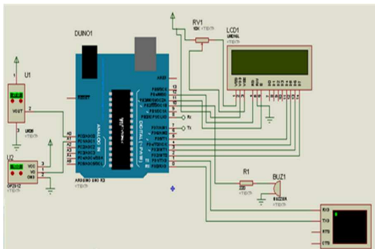
Figure 6: System circuit.
