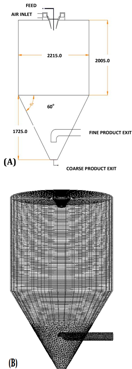
Figure 1. A) Spray-dryer geometry (all dimension in mm) Kieviet[2], B) CFD mesh
