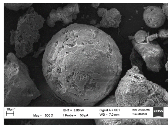
Figure 2: SEM image of raw POFA
