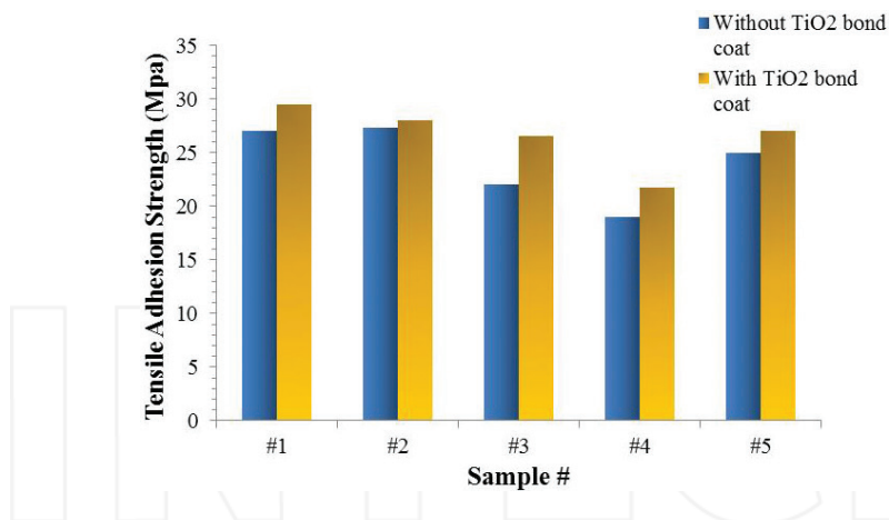
Figure 1. Adhesion strength of the HVSPS-deposited HAp coatings [110].
