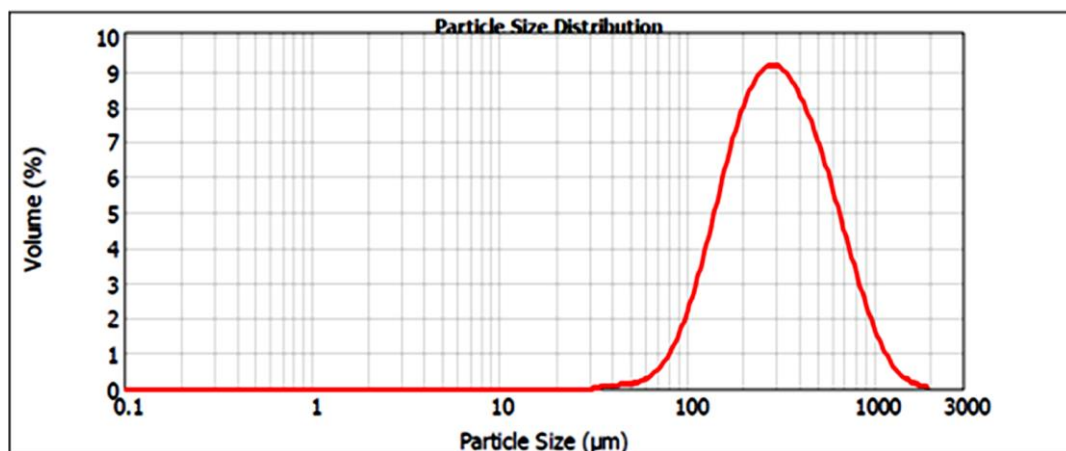
Figure 2. Particle size distribution for SAP.
