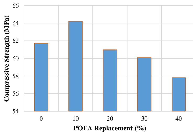
Figure 3. Compressive strength of lightweight aggregate concrete at 28 days.
