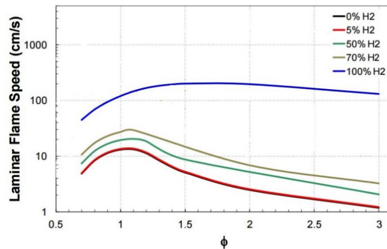
Figure 20. Effect of blending hydrogen in natural gas on the laminar flame speed at 15 kPa and 300 K, extracted from Reference [218].
