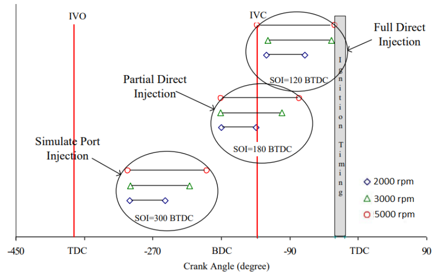
Figure 14. Injection duration for different injection timings for engine speeds 2000 rpm, 3000 rpm, and 5000 rpm [162].
