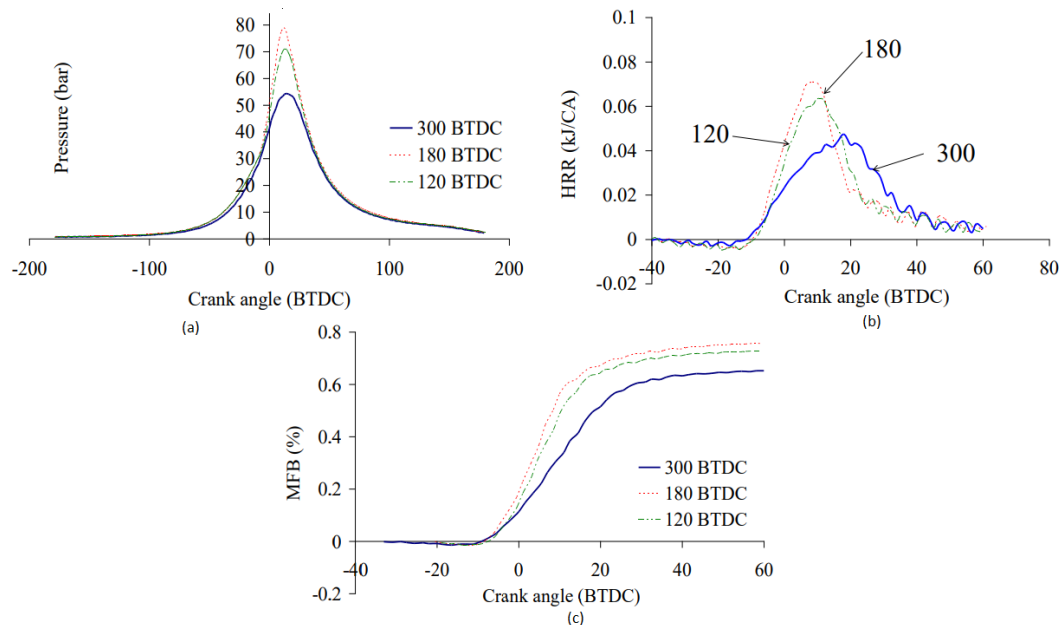
Figure 16. In-cylinder pressure (a), heat release rate (b), and mass fraction burned (c) for different injection timings at an engine speed of 3000 rpm [213].
