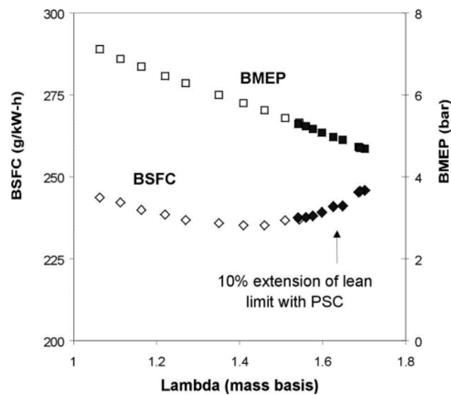
Figure 12. Extension of lean limit by partially stratified charge at 2000 rpm [204].
