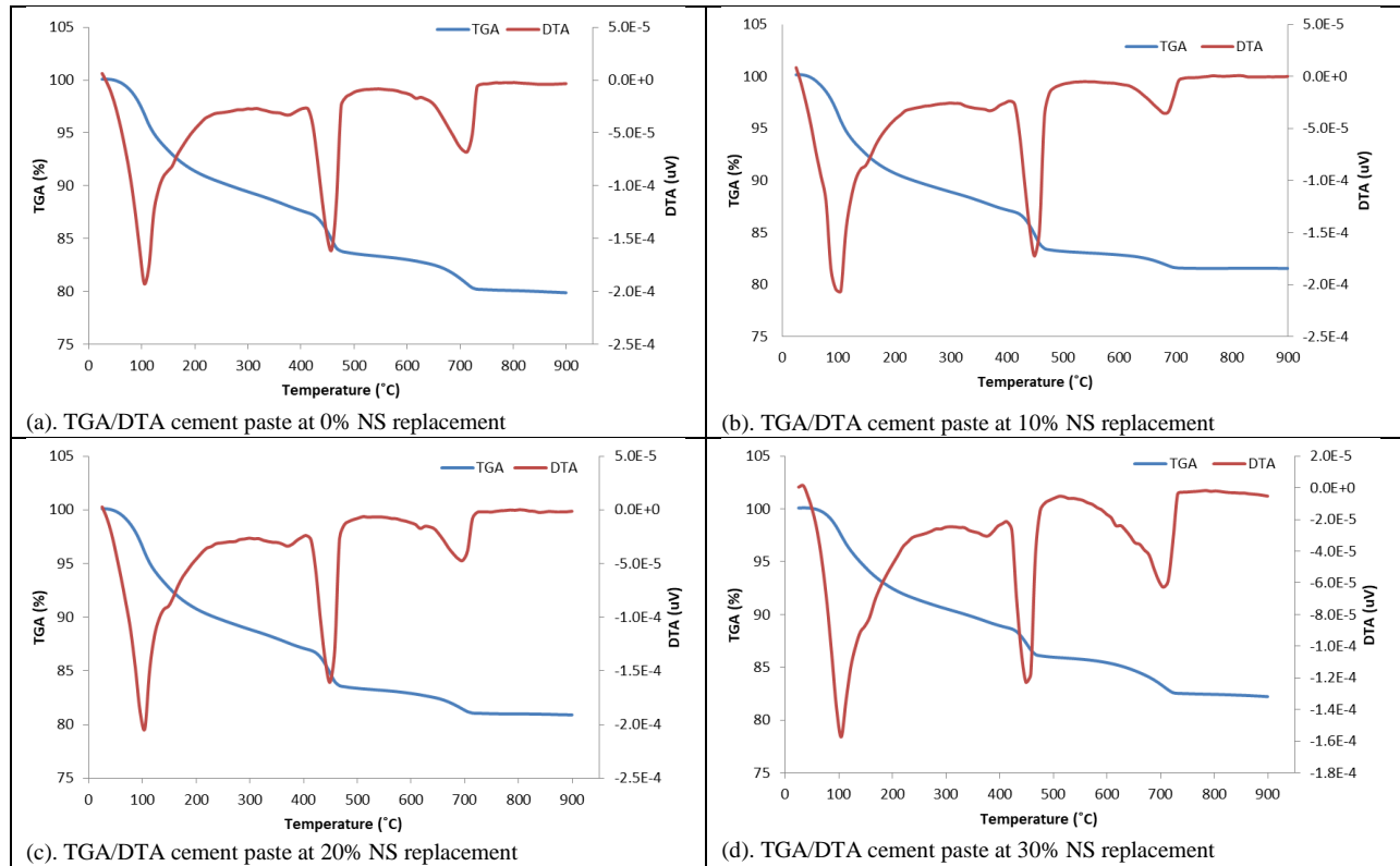
Figure 5 Thermogravimetric and derivative analysis of cement paste with Nano BRHA
