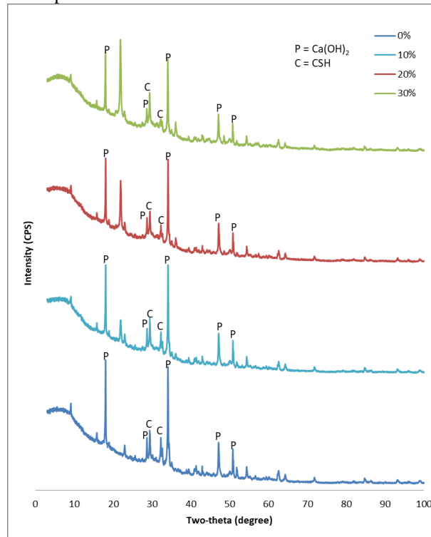
Figure 9 XRD of cement paste at various percentage of nano BRHA replacement
