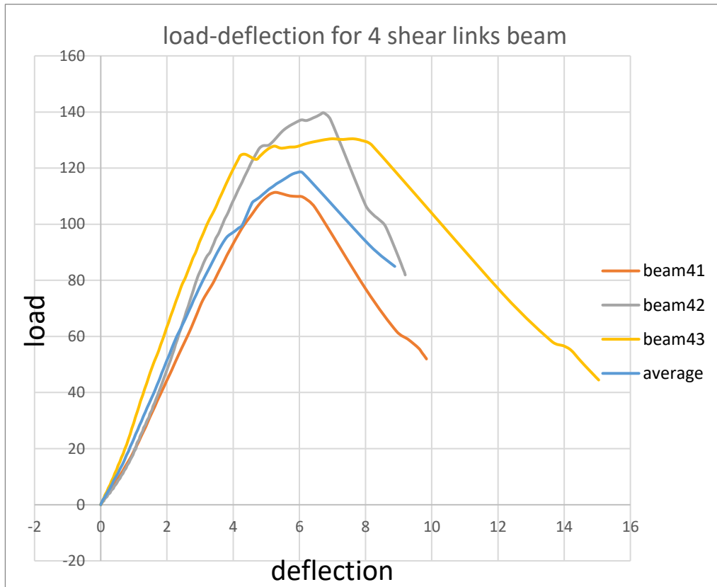
Figure 4.4 Flexural strength of samples with 4 shear links
