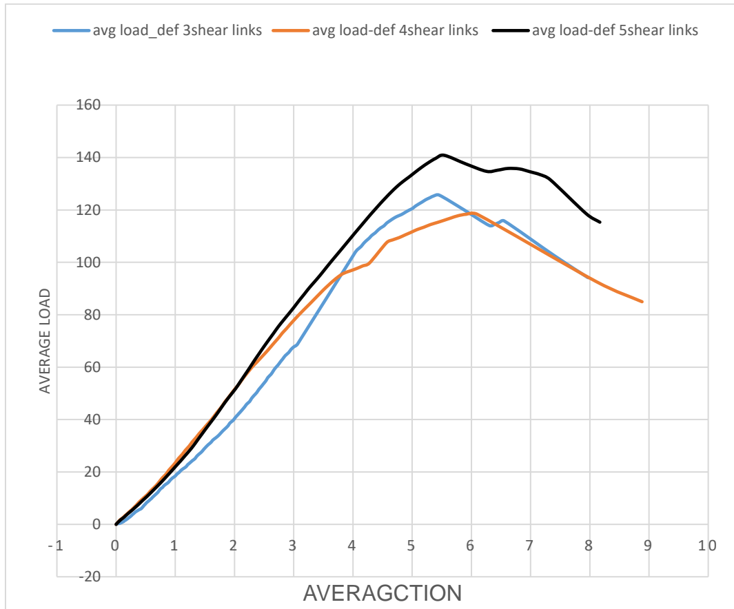
Figure 4.6 Flexural strength average of samples with 3,4 and 5 shear links
