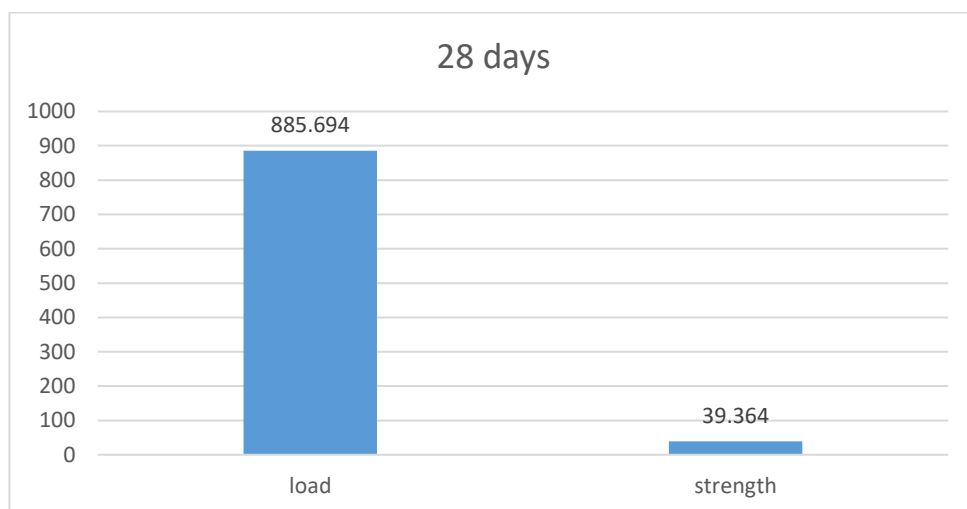
Figure 4.2 Compressive strength and load for cubes tested after 28 days
