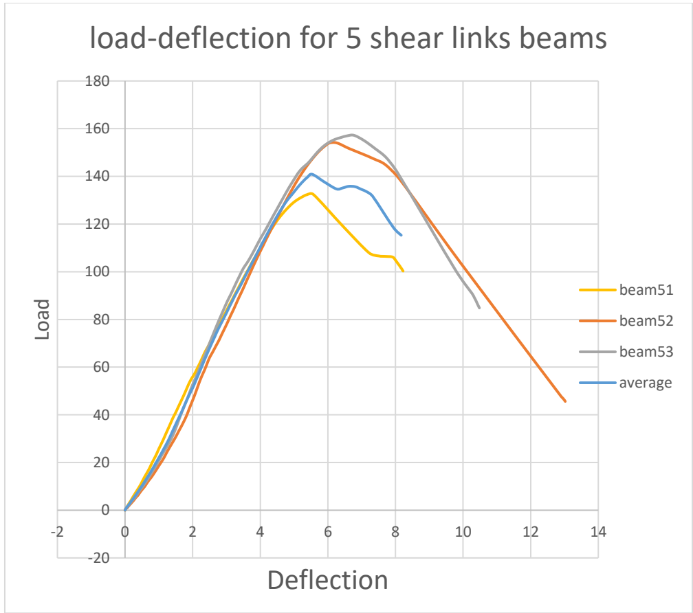
Figure 4.5 Flexural strength of samples with 5 shear links
