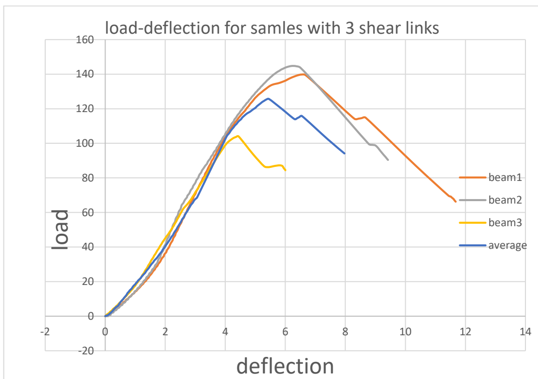
Figure 4.3 Flexural strength of samples with 3 shear links
