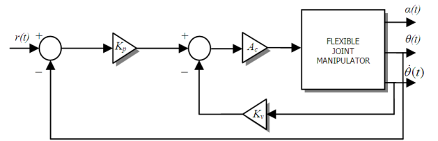
Fig. 2 Collocated PD control structure.
