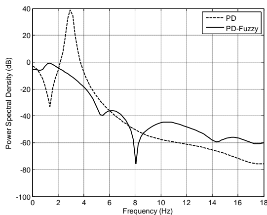
Fig. 8 PSD of deflection angle.
