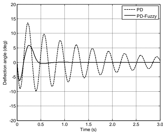
Fig. 7 Deflection angle response.
