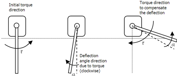
(a) Direction of torque to reduce deflection angle when link moves anti-clockwise
