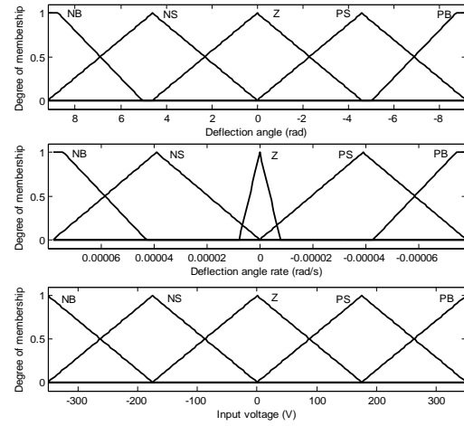
Fig. 4 Membership functions of inputs and output signals.
