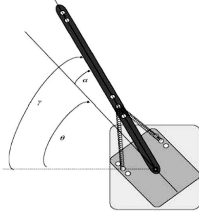
Fig. 1 Description of the flexible joint manipulator system.
