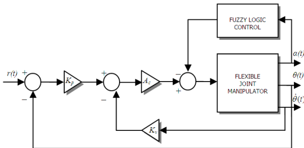
Fig. 3 Collocated PD with non-collocated Fuzzy Logic control structure.
