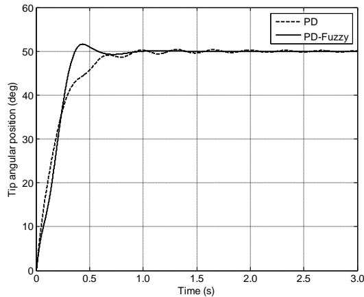
Fig. 6 Tip angular position response.
