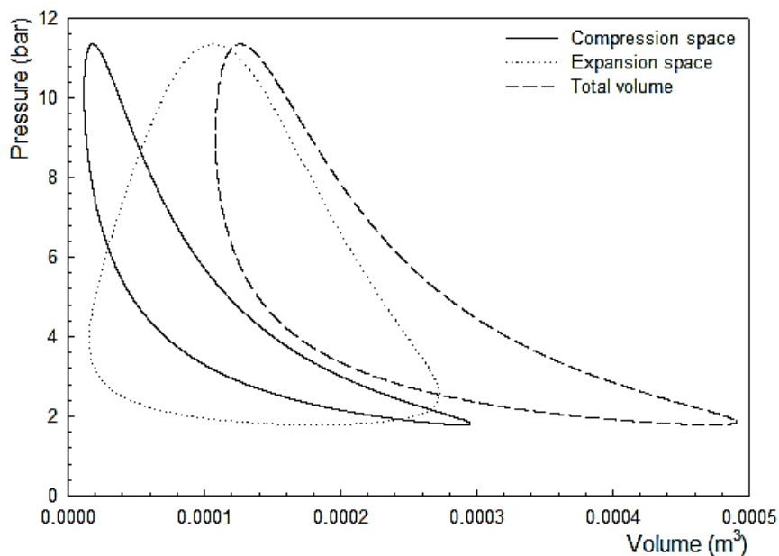
Figure 5. P-V diagram.
