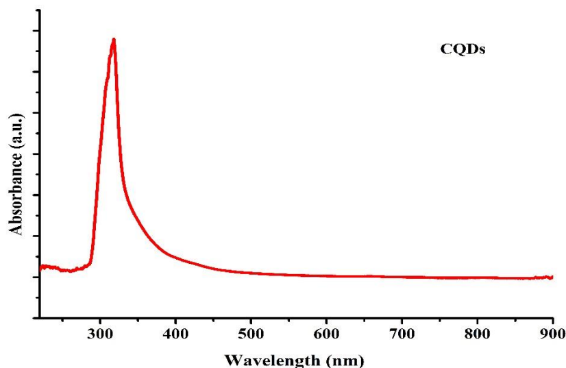
Figure 3: Absorbance spectrum of CQDs
