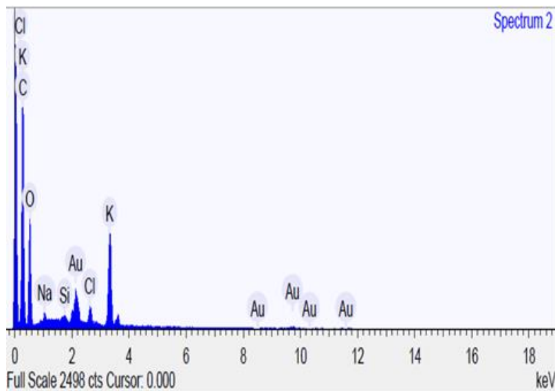
Figure 2: EDX image of CQDs
