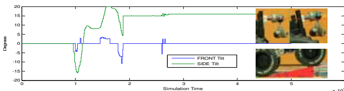
Fig.7. Pitch and roll condition of UGV while climbing
