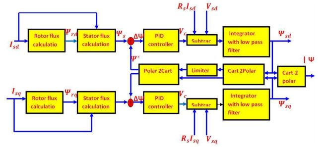
Fig. 3. Block diagram of stator flux estimation.
