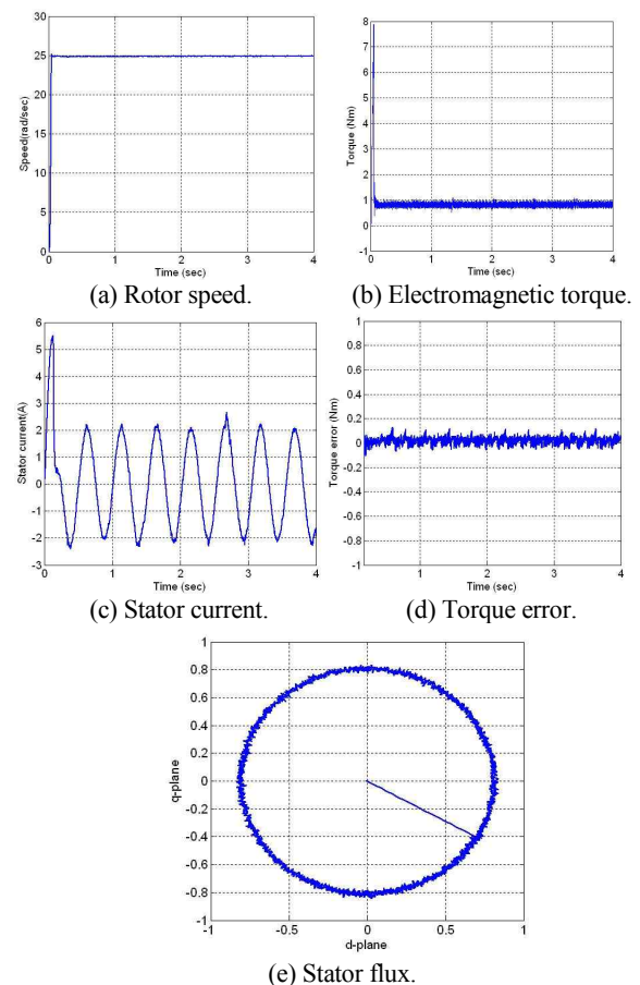
Fig. 13. Results of proposed method (at 25rad/sec).
