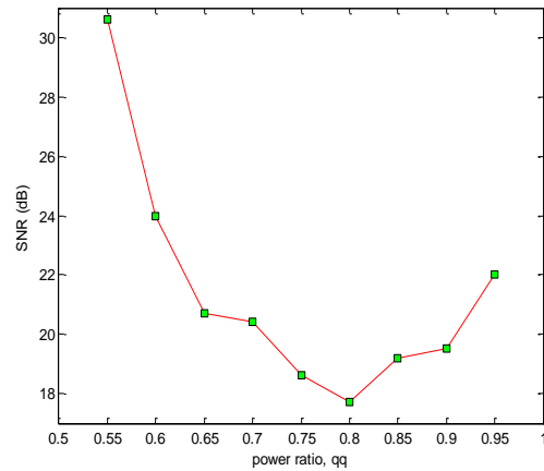
Fig. 3. SNR performance for various power ratios at a target BER of 10^{-3}
