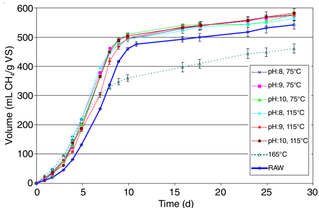
Fig. 1. Methane production from the blend of sewage sludge and petrochemical wastewater with 68:32 mixing ratio without pretreatment and after thermal (165 °C) or thermo-alkaline pretreatments
