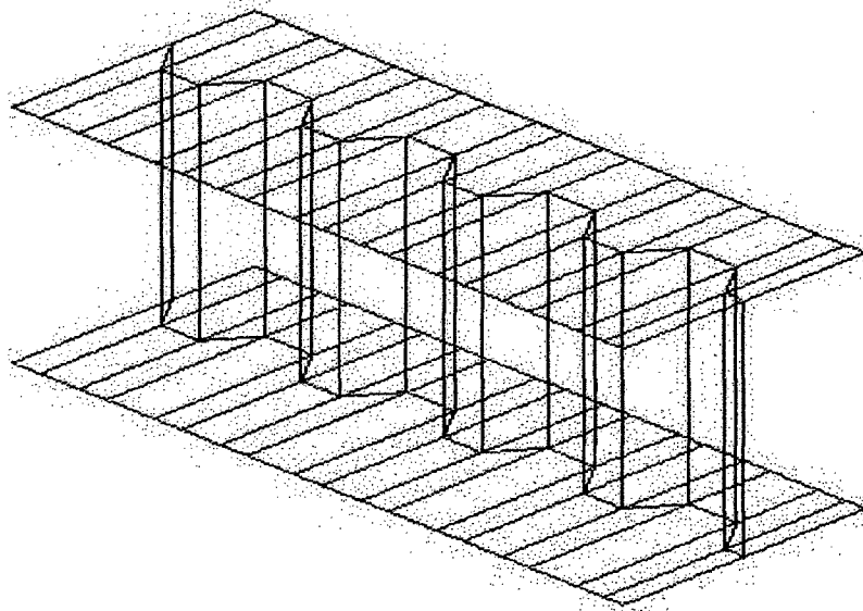
Figure 2.5: Trapezoidal web profiled steel section.
