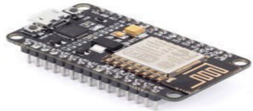
FIGURE 6. NodeMCU.
