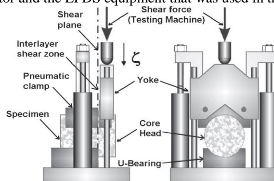
Figure 1. Schematic diagram of the LPDS test device [3]
