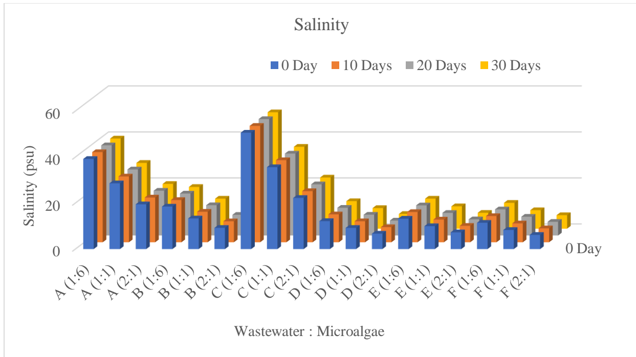
Fig. 6. The Graph representing salinity (psu) of microalgae and wastewater proportions for 30 days treatment period.
