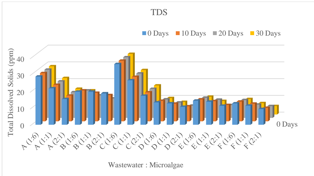
Fig. 5. The total dissolved solids (ppm) of microalgae and wastewater proportions.
