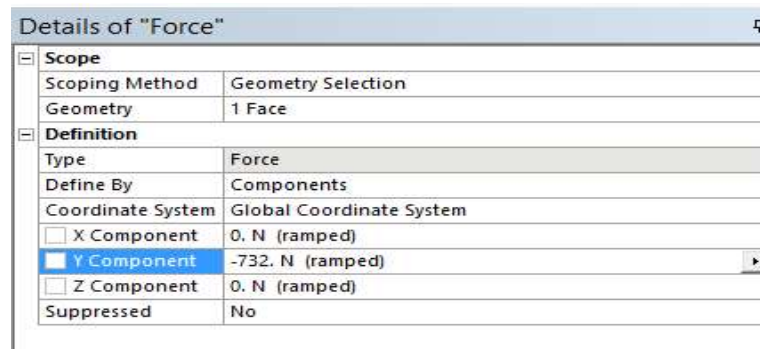
Figure 4. Force applied to the tibial component of ankle implant.
