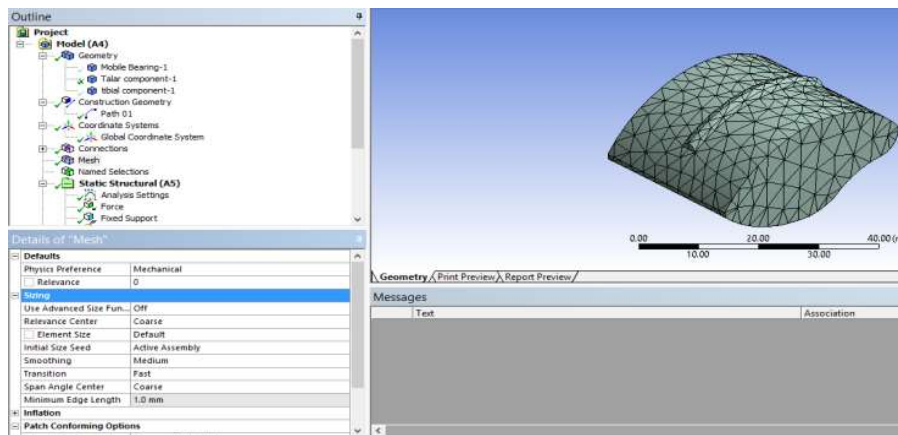
Figure 7. The mesh of mobile bearing using ANSYS software
