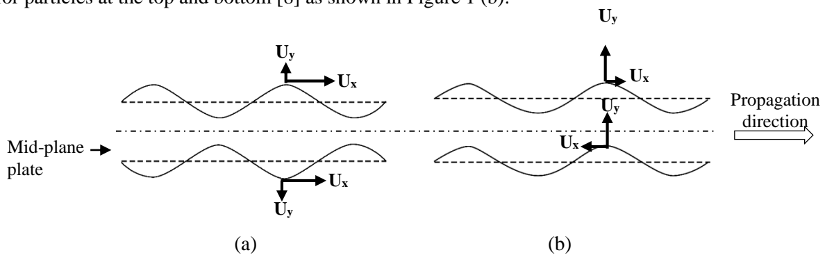
Figure 1. Propagation of the (a) symmetric mode and (b) anti-symmetric mode
