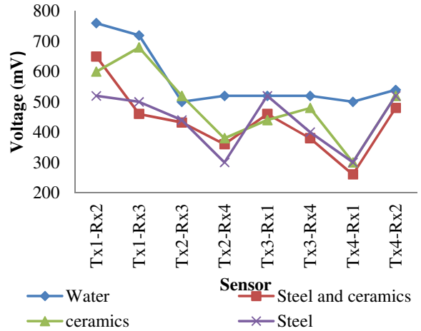
Fig. 3 Graph first highest peak voltage comparison between water with different kinds of materials.
