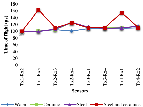
Fig. 4 Graph comparison time of flight between water with different kinds of materials
