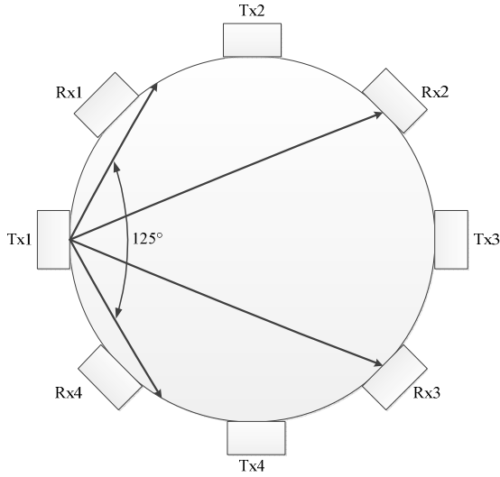
Fig. 1 Sensor arrangement and diverging area
