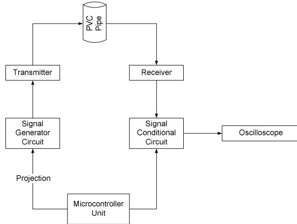
Fig. 2 Ultrasonic tomography system
