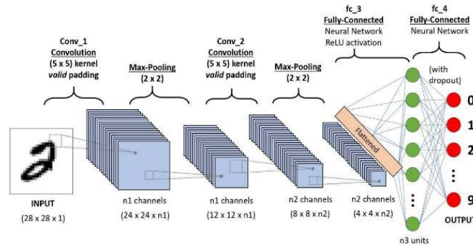
Figure 1. Process of Convolutional Neural Network
