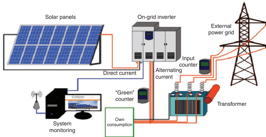
Fig. 3: Grid-connected solar PV system
