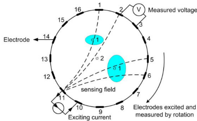
Figure 1. Operating principle of ERT [12]
