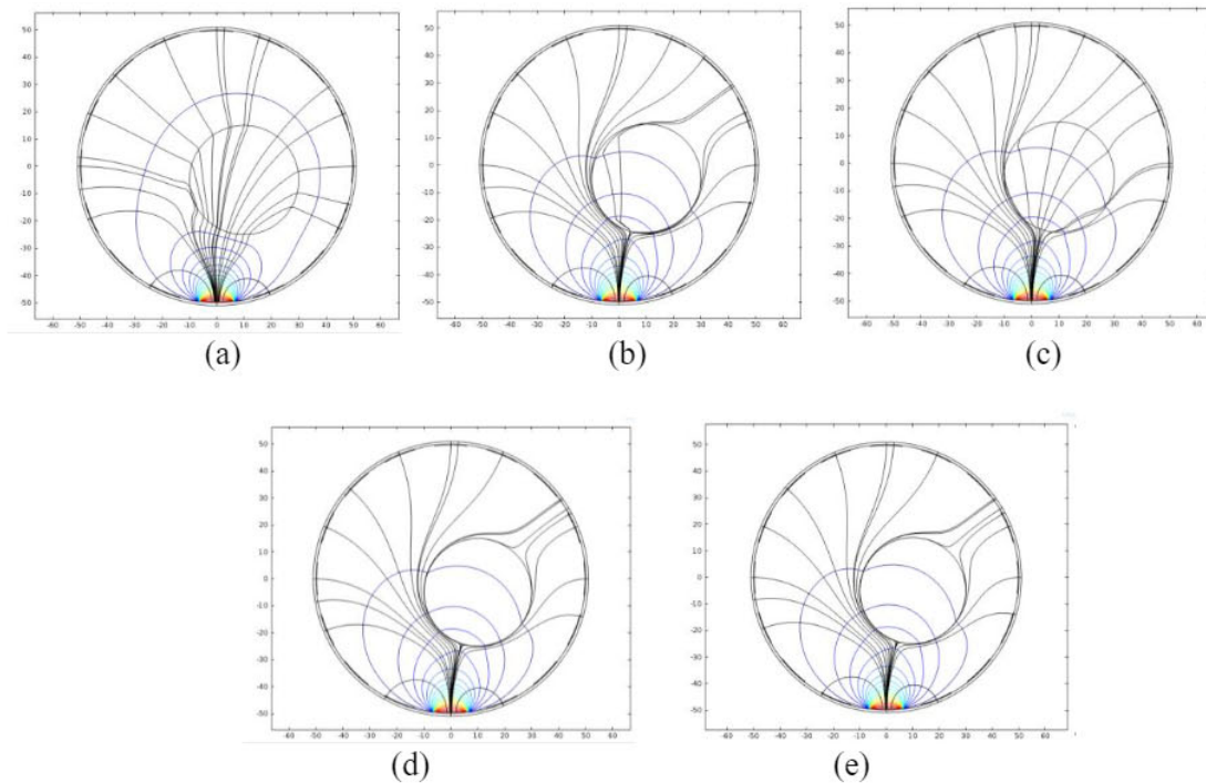
Figure 8. Effect of different conductivities, \sigma on the contour of electric potential with current density streamlines (a) \sigma = 3.477 \times 10^7 S/m, (b) \sigma = 1 \times 10^{-4} S/m, (c) \sigma = 1 \times 10^{-3} S/m, (d) \sigma = 1 \times 10^{-14} S/m, (e) \sigma = 5 \times 10^{-15} S/m
