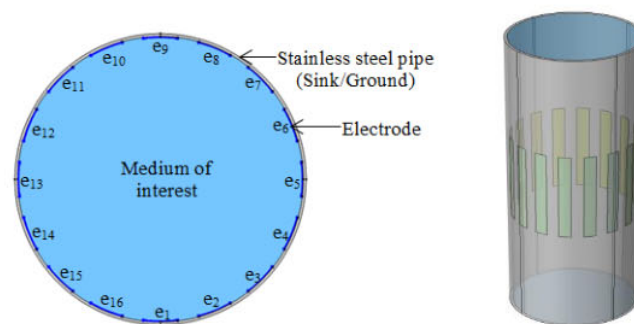
Figure 3. Cross sectional view and 3D ERT model developed in COMSOL
