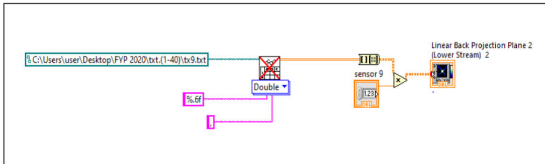
Figure 6. Single view of linear back projection algorithm
