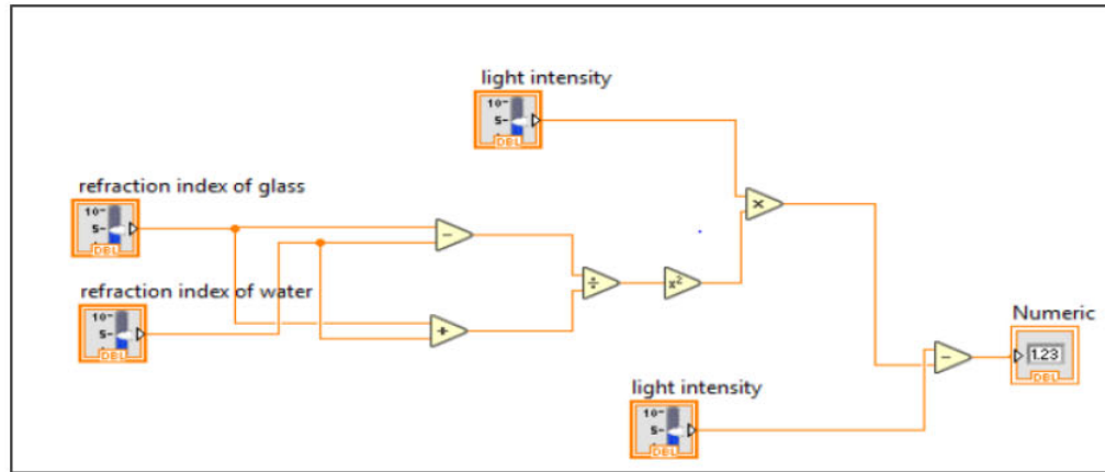
Figure 5. LabVIEW coding for light reflection calculation
