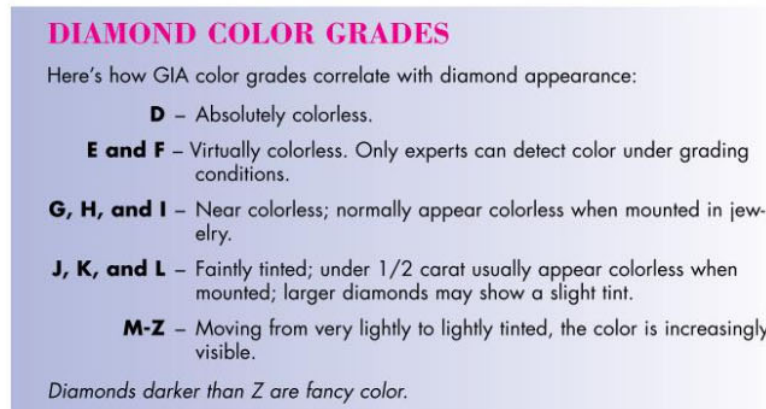
Figure 2. The diamond colour grade based on GIA [4].
