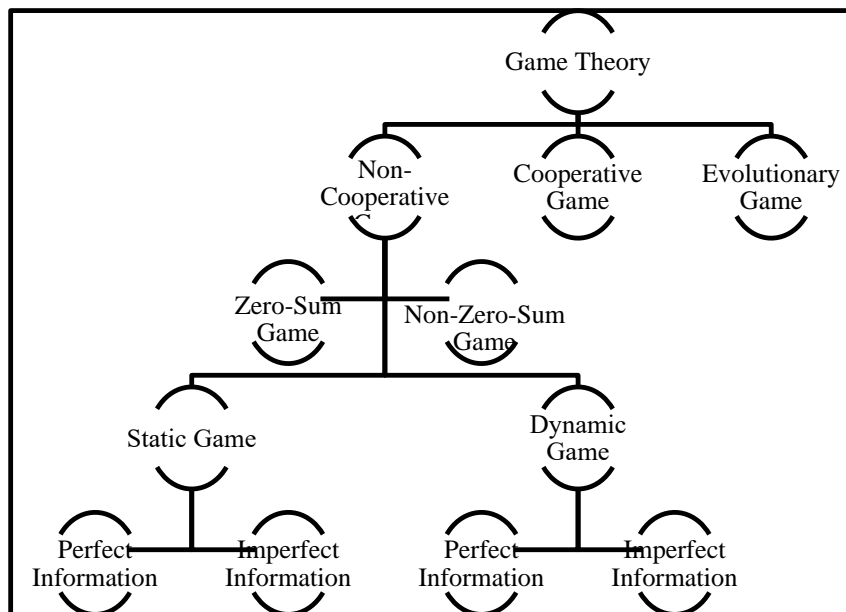
Figure 1. The main classification of game theory techniques.
