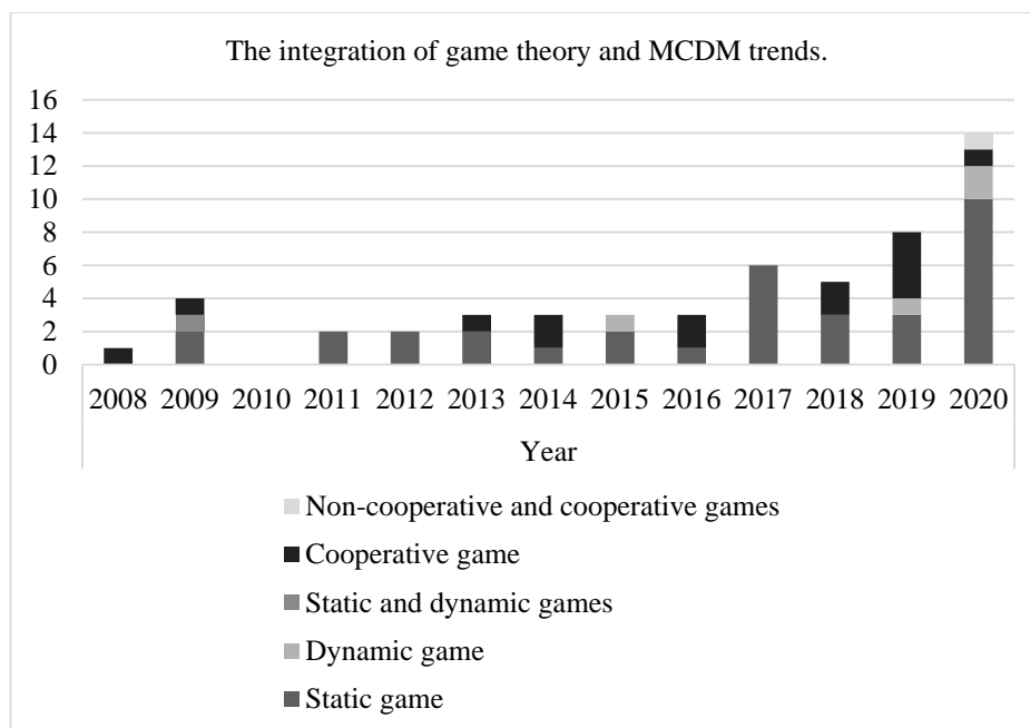
Figure 2. The integration of game theory and MCDM trends.
