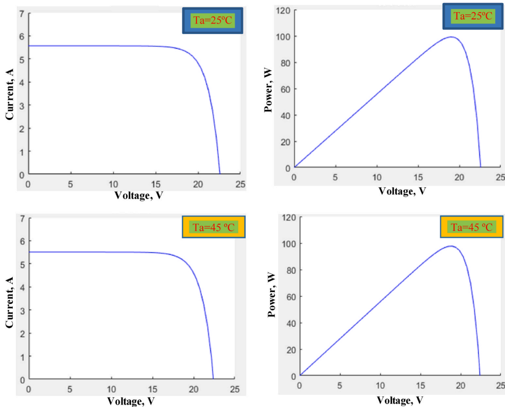
Fig. 7. Volt-current and output power with thermal protective film at STC 25 °C and 45 °C.
