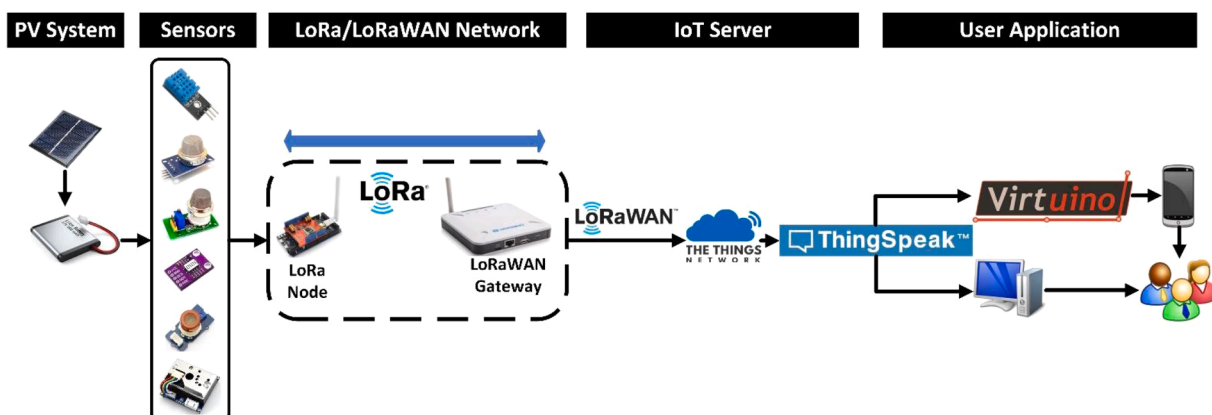
Fig. 3. Overall system architecture.
