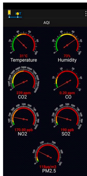
Fig. 19. Virtuino GUI of LoRaWAN-IoT-AQMS.
