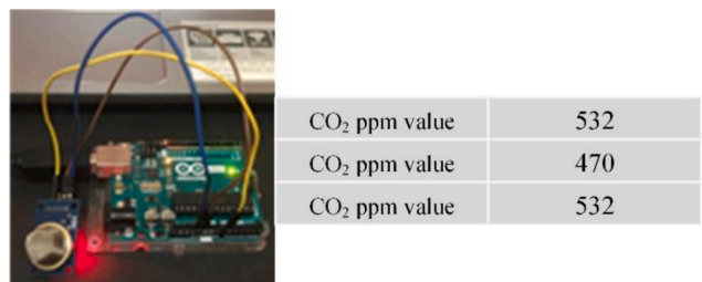
Fig. 6. Calibration of MQ-135 sensor for CO 2 .
