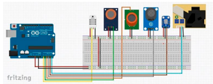
Fig. 5. Circuit design.
