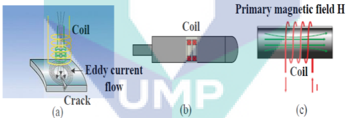
Figure 3: Typical EC probes; (a) Pancake type coil, (b) Bobbin type coil, (c) Encircling type coil
