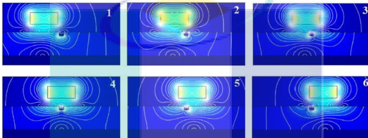
Figure 7: A magnetic model of the MP-GMR probe
