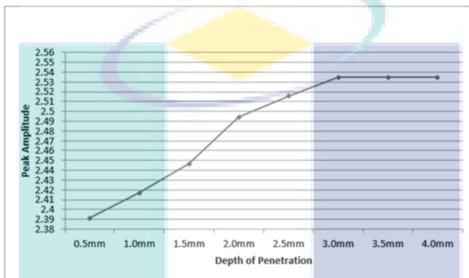
Figure 13: Full reading for signal for all depth slots of mild steel block width 1mm
