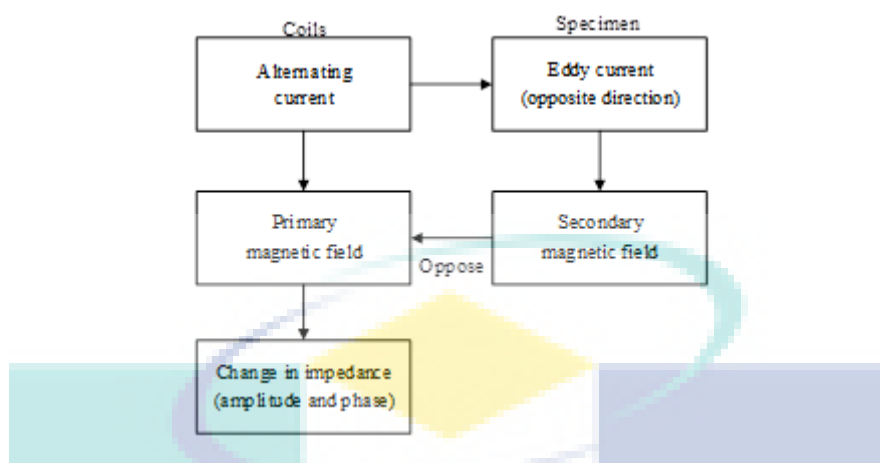
Figure 1: Principle diagram for eddy current testing
