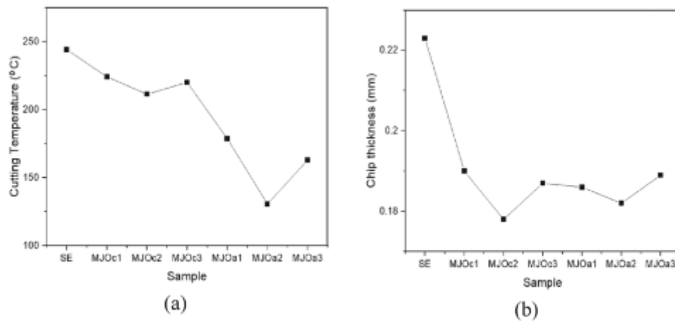
Fig. 1 (a) Cutting temperature (b) chip thickness
