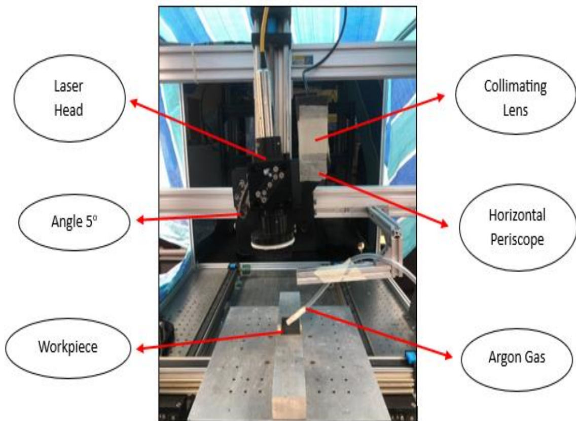
Figure 1. Experimental setup of Pulse Laser Welding
