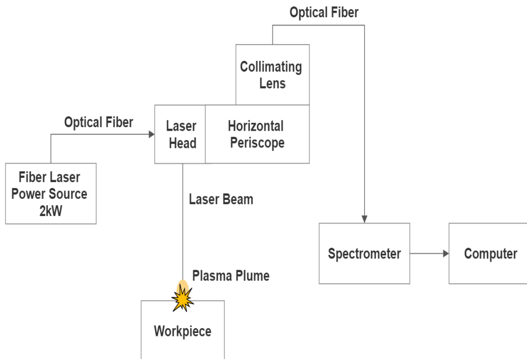
Figure 2. Schematic diagram of data acquisition setup.
