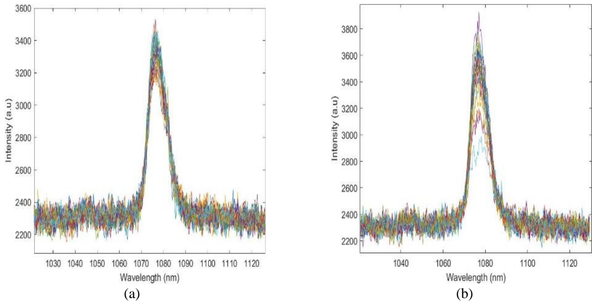
Figure 4. Pulse optical signal acquired during pulse mode laser welding with parameters set as in (a) Group 1 (b) Group 2
