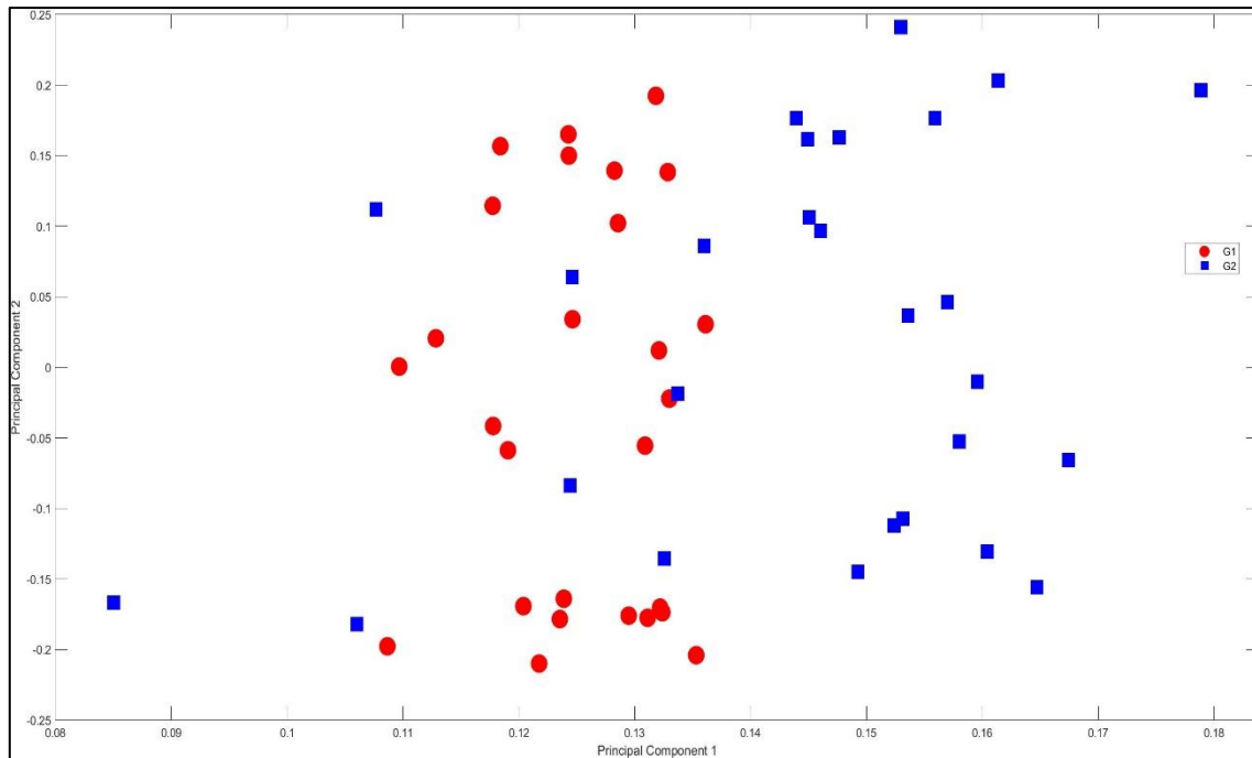
Figure 5. Scatter diagram resulting from the employment of PCA.
