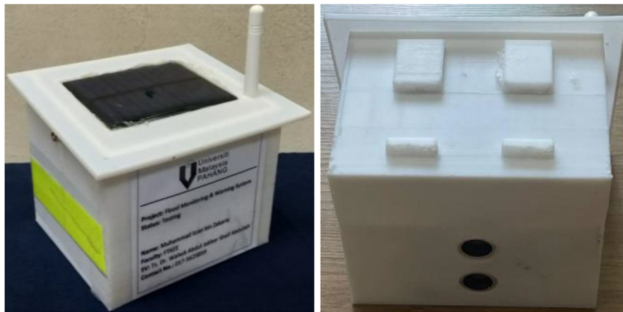
Fig. 4. LoRaWAN FMWS exterior view.
