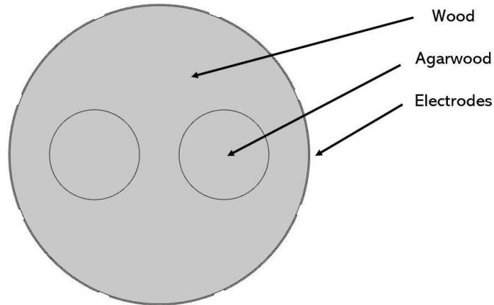
Figure 2. 2-Dimensional geometry model for ECT
