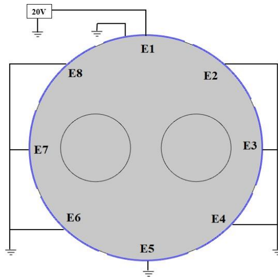
Figure 3. Actual set up signal of ECT model
