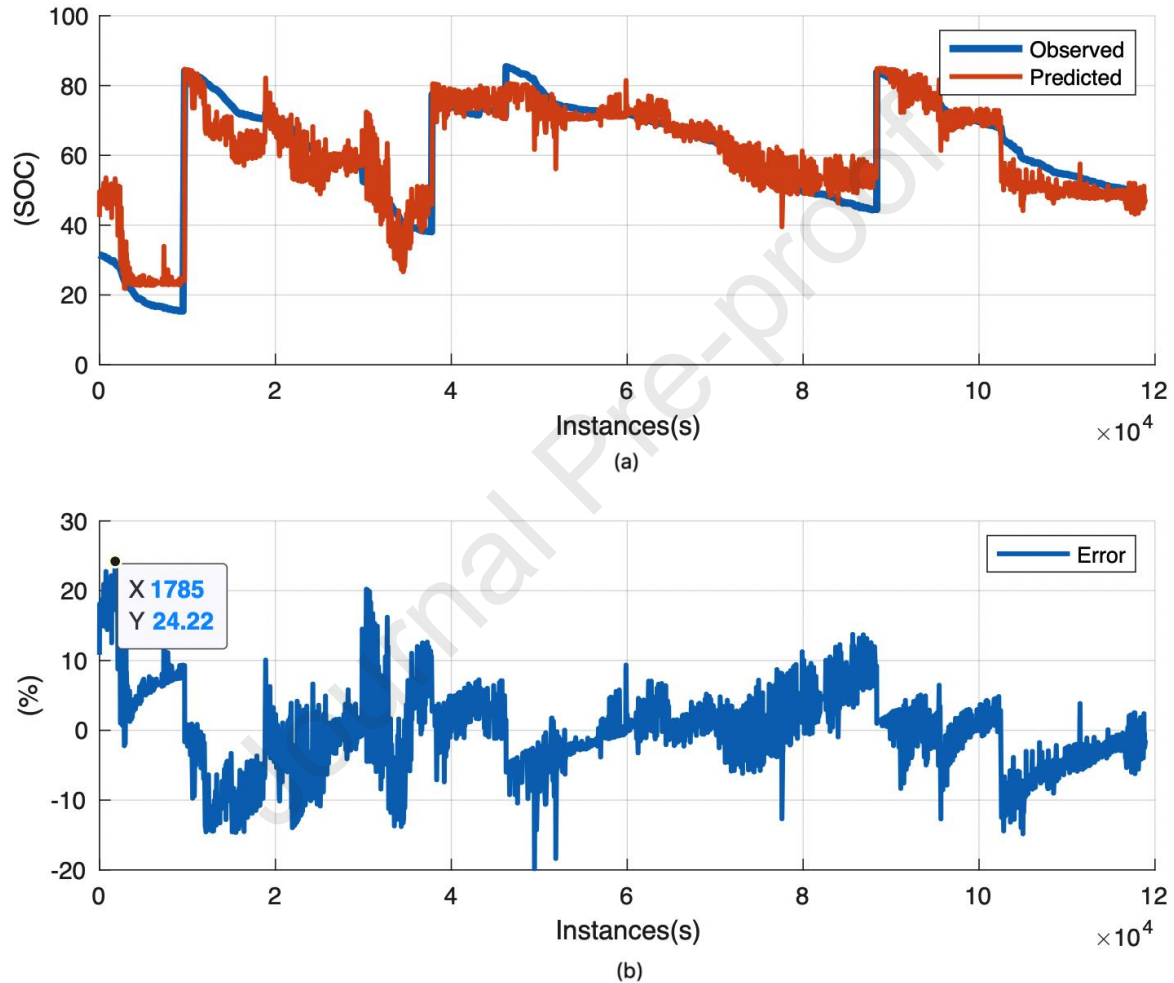
Fig. 3. Results of the (a) SOC estimation by RF for the testing data, (b) Error between actual and predicted.
