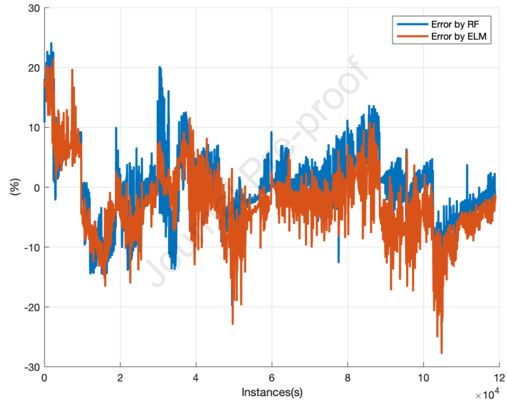
Fig. 6. Error comparison between RF and ELM for SOC estimation.
