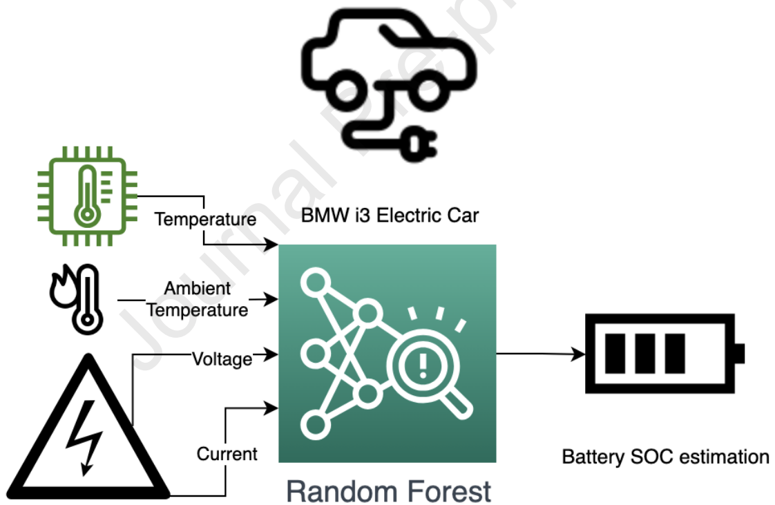
Fig. 1. SOC estimation using Random Forest (RF)
