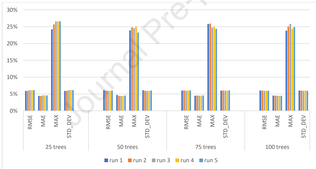
Fig. 2. Performance metrics for various configuration of trees in RF model for SOC estimation.
