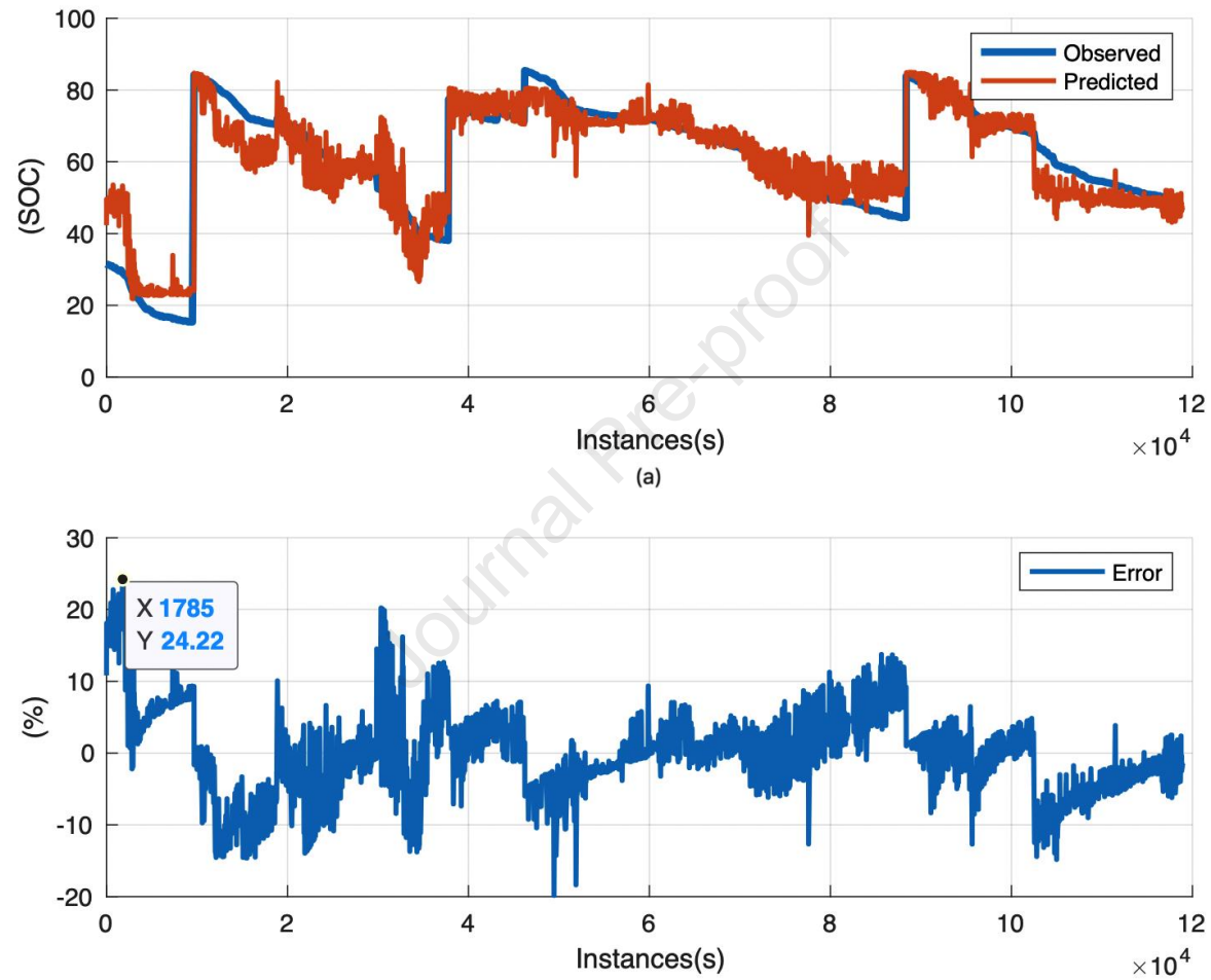
Fig. 3. Results of the (a) SOC (b) estimation by RF for the testing data, (b) Error between actual and predicted.
