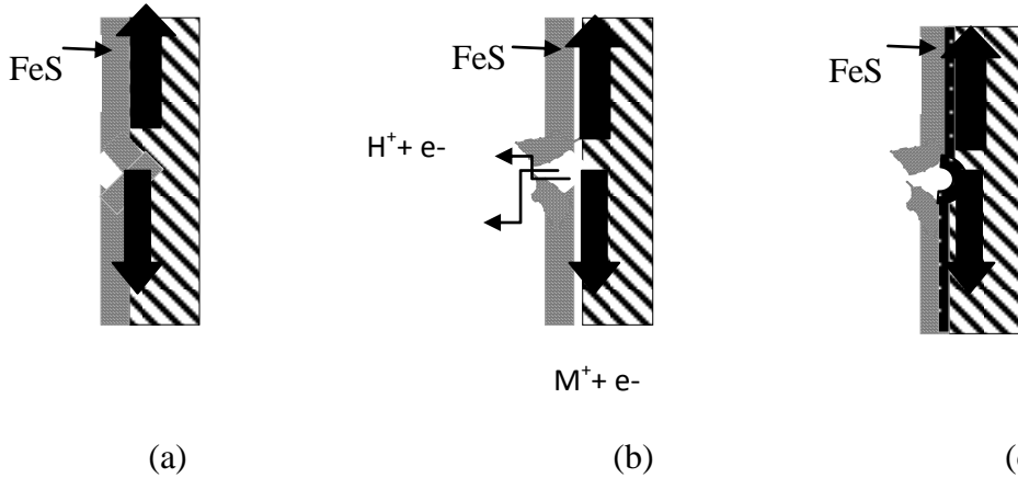
Figure 2. Models of film formation and film dissolution assumed at crack tip during corrosion process under stress condition.
