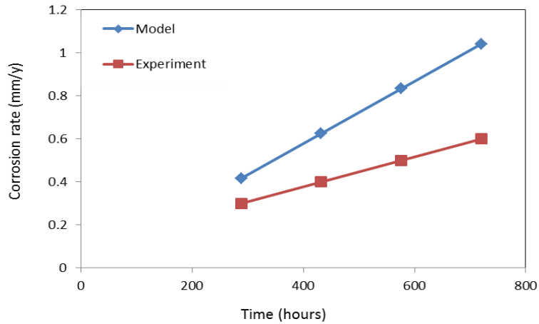
Figure 6. Comparison between the model to Irawan's experiment (in 1 % of H 2 S saturated solutions at temperature 40°C, pH 4, total pressure 1bar )
